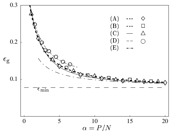
FIG. 1. Linear target rule corrupted by additive Gaussian noise ( \langle \eta \rangle = 0 , \langle \eta^2 \rangle = 1/16 ) and learned using different kernels. The curves are the theoretical prediction; symbols show simulation results for N = 600 with Gaussian inputs and error bars are approximately the size of the symbols. (A) Gaussian kernel, \Phi(z) = e^{-kz} with k = 2/3 . (B) Wiener kernel given by the nonanalytic function \Phi(z) = e^{-c\sqrt{z}} . We chose c \approx 0.065 so that the theoretical prediction for this case coincides with (A). (C) Gaussian kernel with k = 1/20 , the influence of the parameter change on the learning curve is minimal. (D) Perceptron, \phi(z) = z . Above \alpha_c \approx 7.5 vanishing training error cannot be achieved and the SVM is undefined. (E) Kernel invariant asymptote for (A,B,C).
