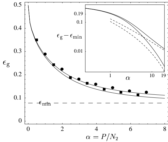
FIG. 2. A noisy quadratic rule ( T_1 = 0, T_2 = 1 ) learned using the Gaussian kernel with k = 1/20 . The upper curve (simulations \bullet ) is for additive Gaussian noise as in Fig. 1. The lower curve (simulations \blacksquare ) is for binary noise, \eta \pm s with equal probability. We chose s \approx 0.20 so that the value of \epsilon_{\min} is the same for the two noise processes. The inset shows that \epsilon_g decays as 1/\alpha for Gaussian noise, whereas an exponential decay is found in the binary case. The dashed curves are the kernel invariant asymptotes. The simulations are for N = 90 with Gaussian inputs, and standard errors are approximately the size of the symbols.
